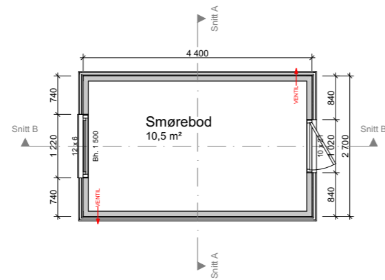
Plan bod
